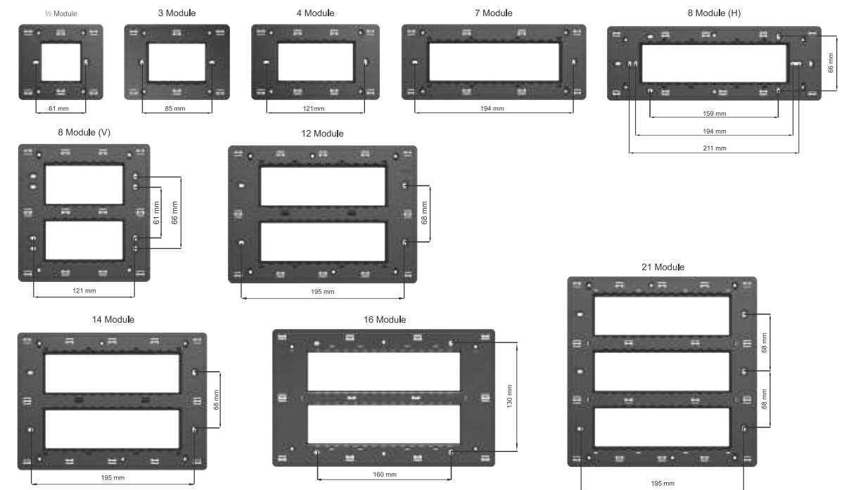
FRINTON FAROS BASE PLATE (Dimensions in mm)
