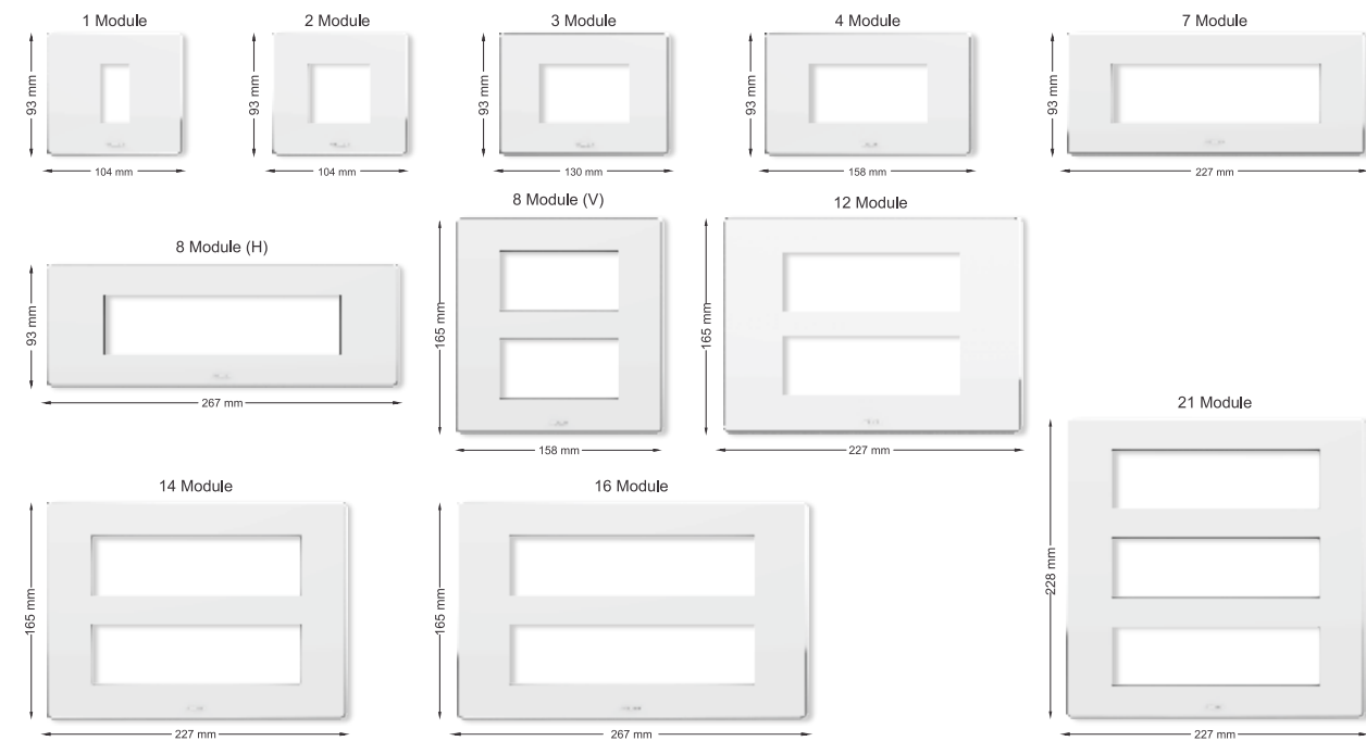
FRINTON FAROS COVER PLATE WITH SIDE FRAME (Dimensions in mm)
